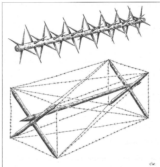
afb.26 Friese ruiters
