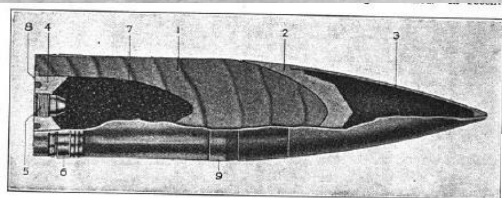
Plate 58. Armor-Piercing Projectile
